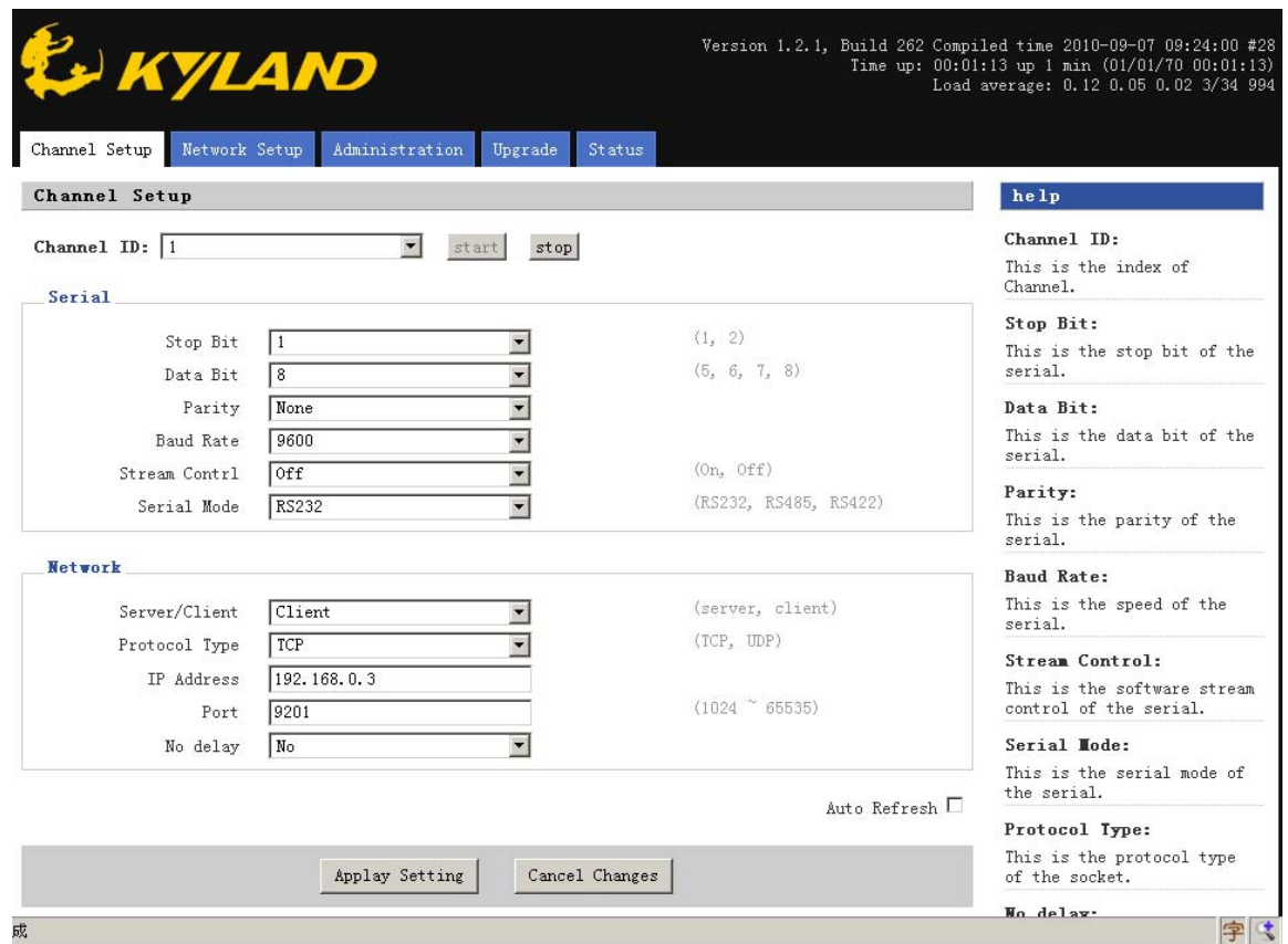
Figure 4-6: TCP Client settings
