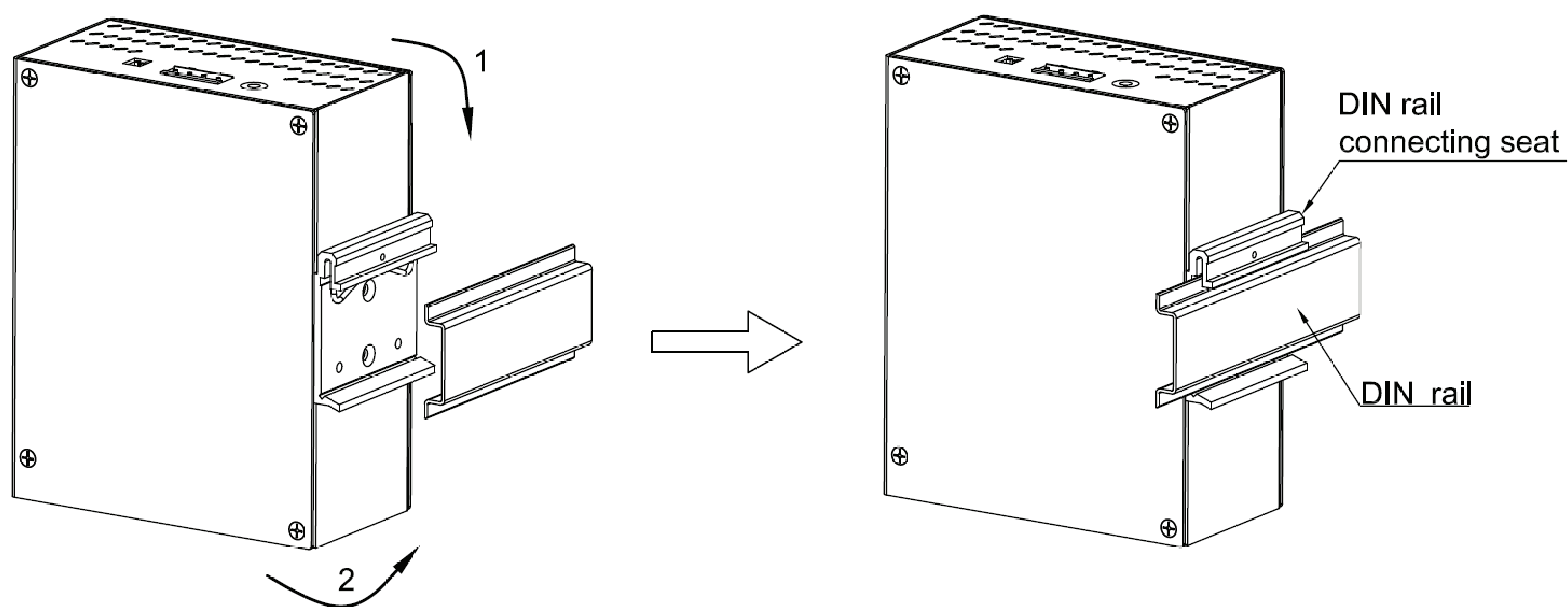
Figure 5 DIN-Rail Mounting
