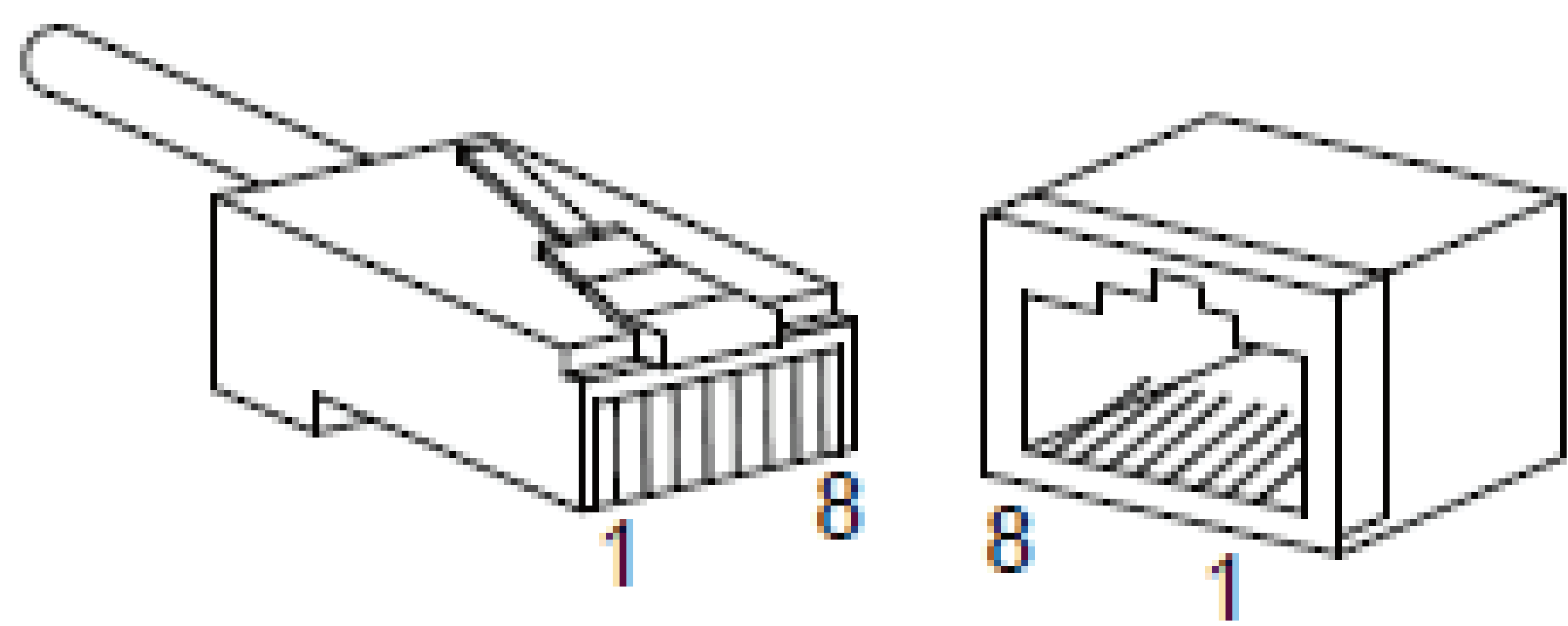
Figure 7 RJ45 Port
