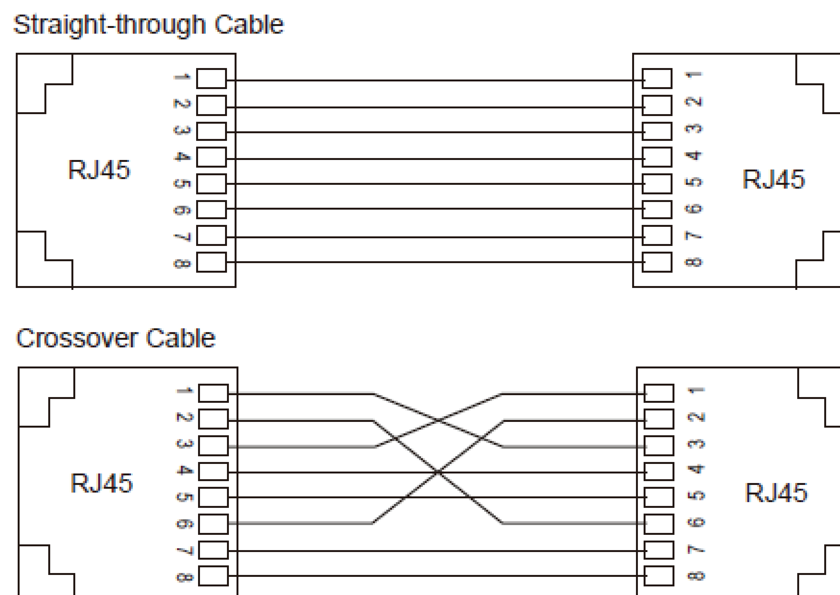
Figure 8 Connection Using Straight-through/Cross-over Cable
