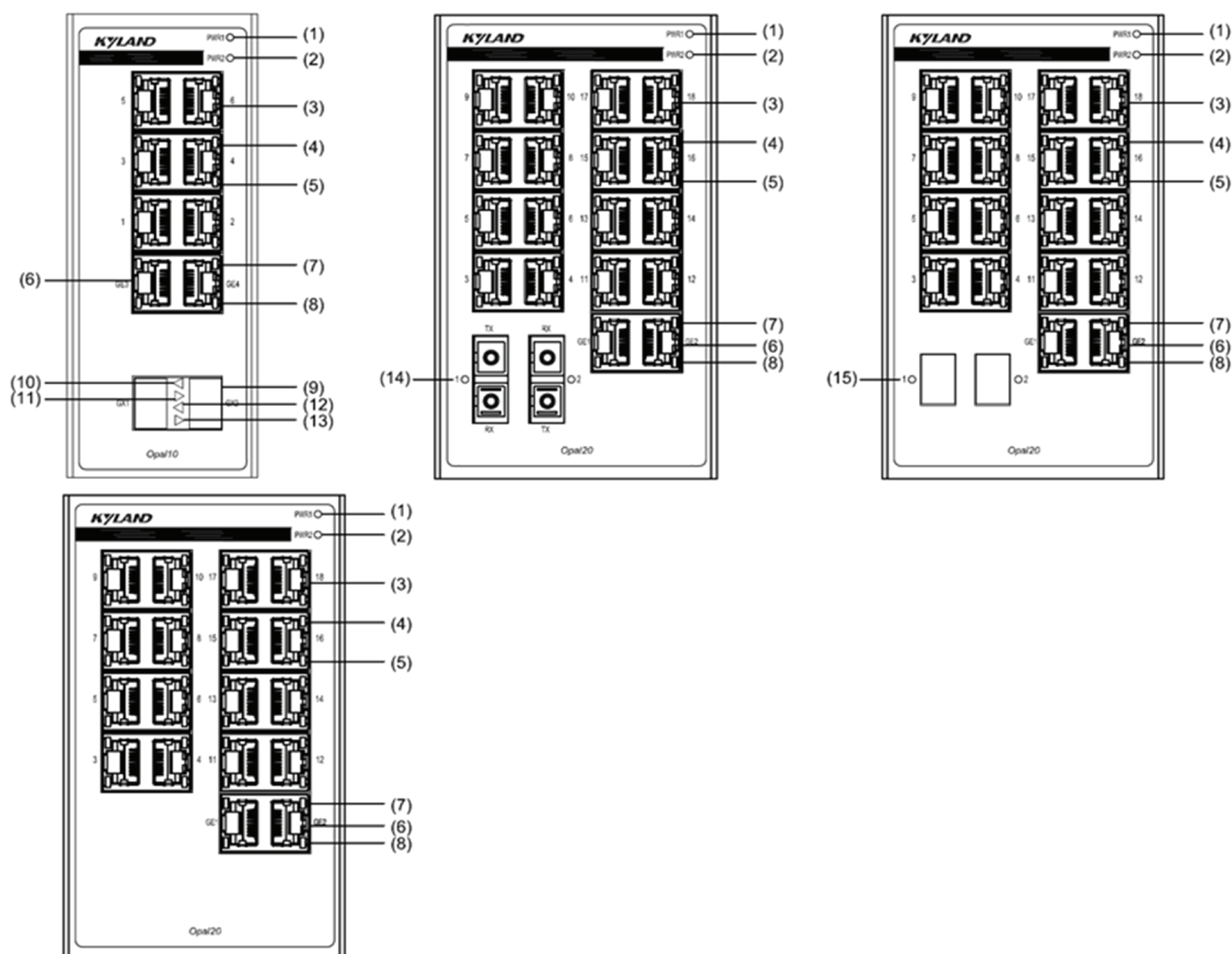
Figure 1 Front Panel
