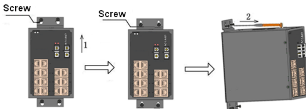
Figure 9 Panel Dismounting
