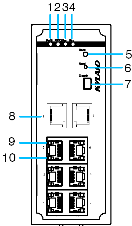
Figure 4 Front Panel 4
