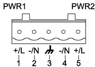
Figure 18 5-pin 5.08mm-spacing Plug-in Terminal Block
