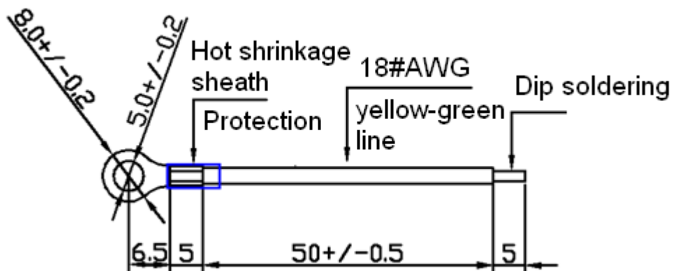
Figure 20 18#AWG Yellow-Green Line (Unit: mm)
