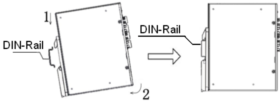
Figure 8 DIN-Rail Mounting
