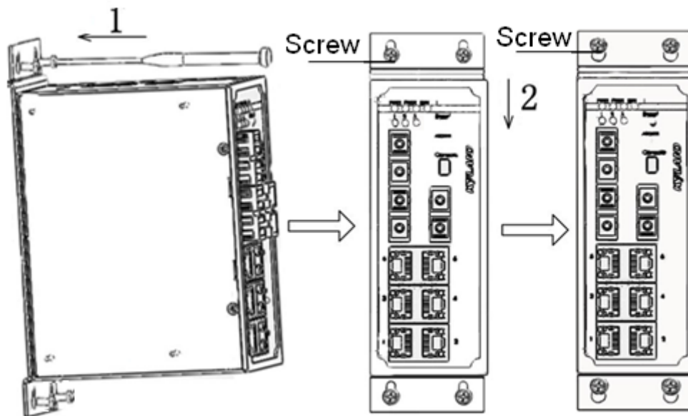
Figure 10 Panel Mounting
