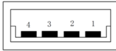
Figure 17 USB Connector
