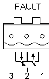
Figure 22 3-Pin 5.08mm-Spacing Plug-In Terminal Blocks
