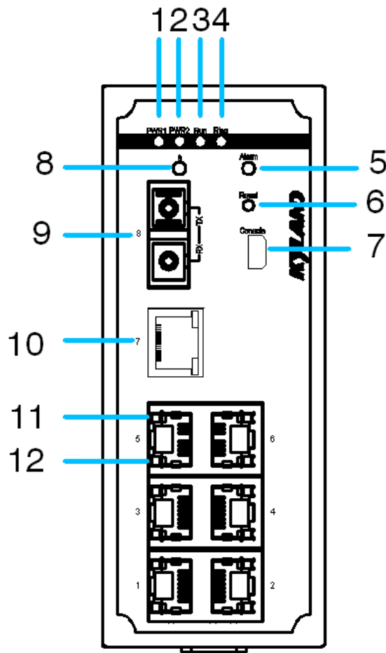
Figure 3 Front Panel 3
