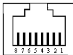
Figure 12 RJ45 Port
