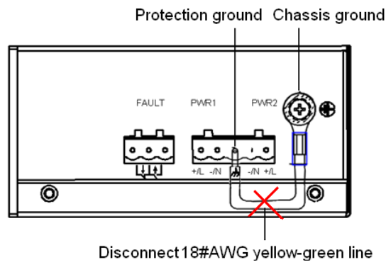
Figure 21 Disconnect 18#AWG Yellow-Green Line (Unit: mm)
