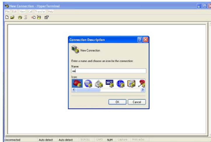
Figure 24 New Connection
