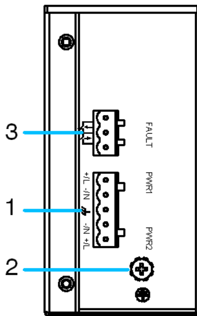
Figure 5 Top Panel
