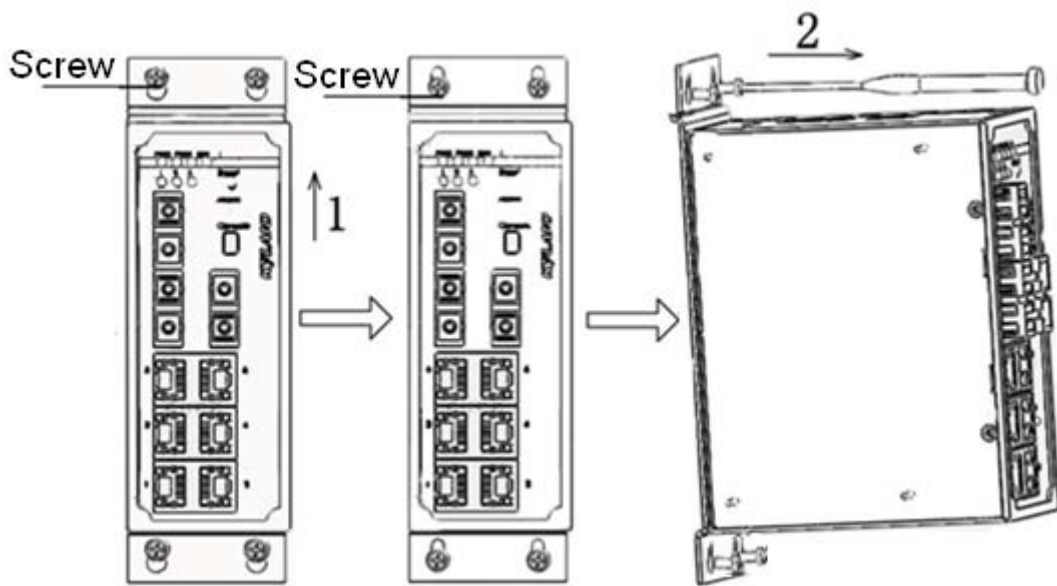
Figure 11 Dismounting
