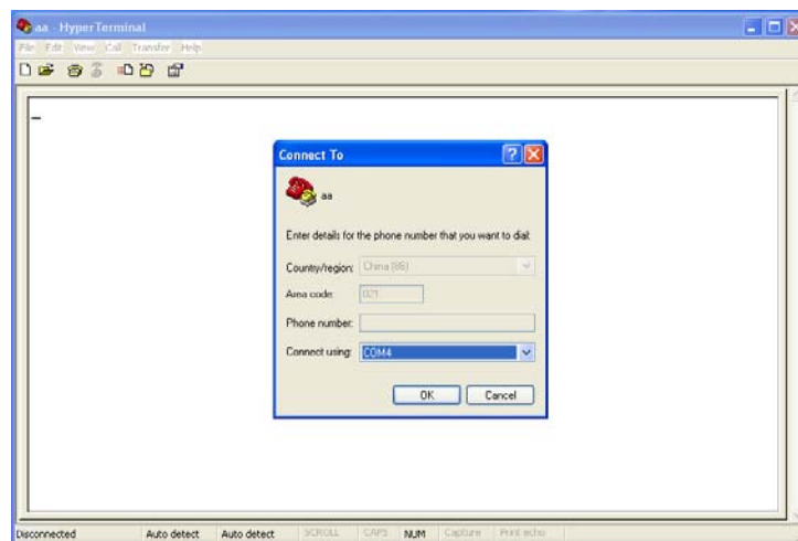
Figure 25 Choose Port
