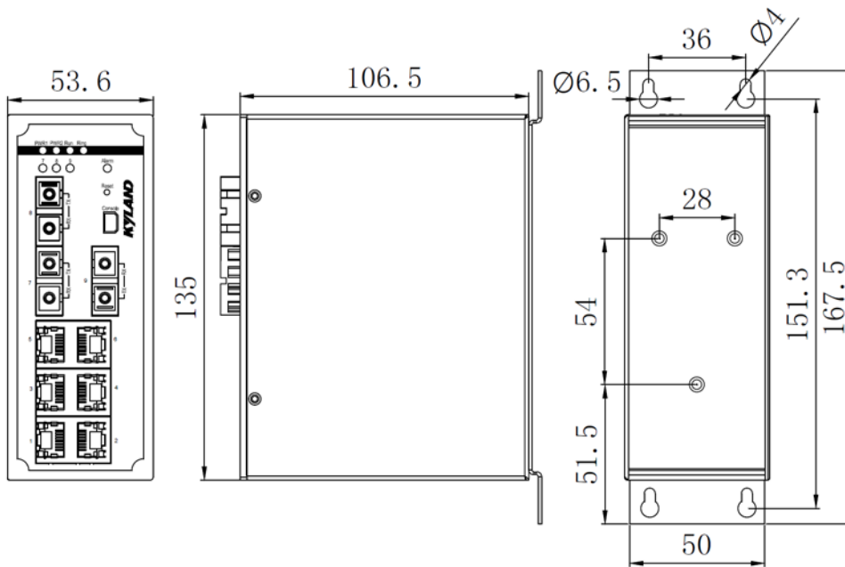
Figure 7 Panel Mounting Dimension
