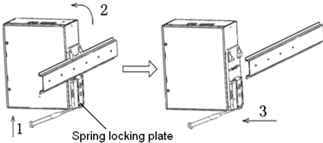
Figure 9 Dismounting
