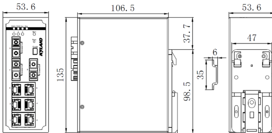
Figure 6 DIN-Rail Mounting Dimension
