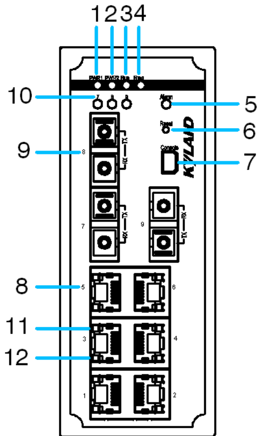
Figure 1 Front Panel 1
